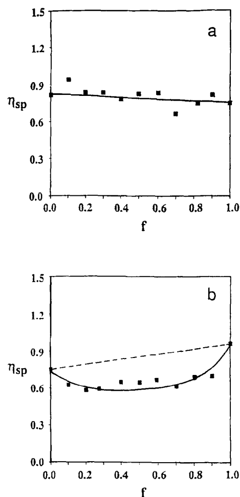
Fig. 3. Specific viscosity (measured at 20°C and 50 s -1 as \dot{\gamma} was increased) for dilute solutions of iota carrageenan and LBG in (a) 100 mM KCl; and (b) 90 mM CaCl 2 ; f denotes the LBG content expressed as a fraction of the total polymer concentration; the concentrations (% w/w) of the individual polymer solutions were: (a) 0.063 LBG, 0.063 carrageenan; and (b) 0.069 LBG, 0.047 carrageenan.
