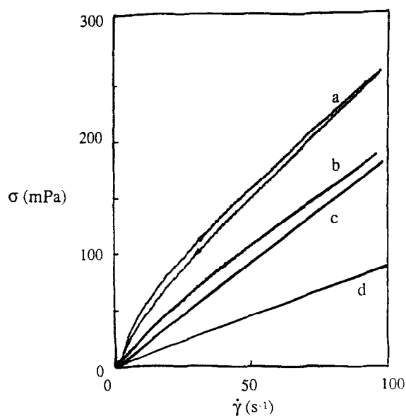
Fig. 1. Flow curves (20°C) of shear stress ( \sigma ) vs shear rate ( \dot{\gamma} ) for stock solutions ( \eta_{sp} \approx 1 ) of xanthan (0.008% w/w) and LBG (0.08% w/w) dialysed together against 10 mM KCl, and for an illustrative mixture with a xanthan:LBG ratio of 7:3. (a) mixed solution (arrows indicate increasing and decreasing \dot{\gamma} ); (b) xanthan alone; (c) LBG alone; (d) dialysate; traces for (b), (c) and (d) gave close superposition on increasing and decreasing \dot{\gamma} .
