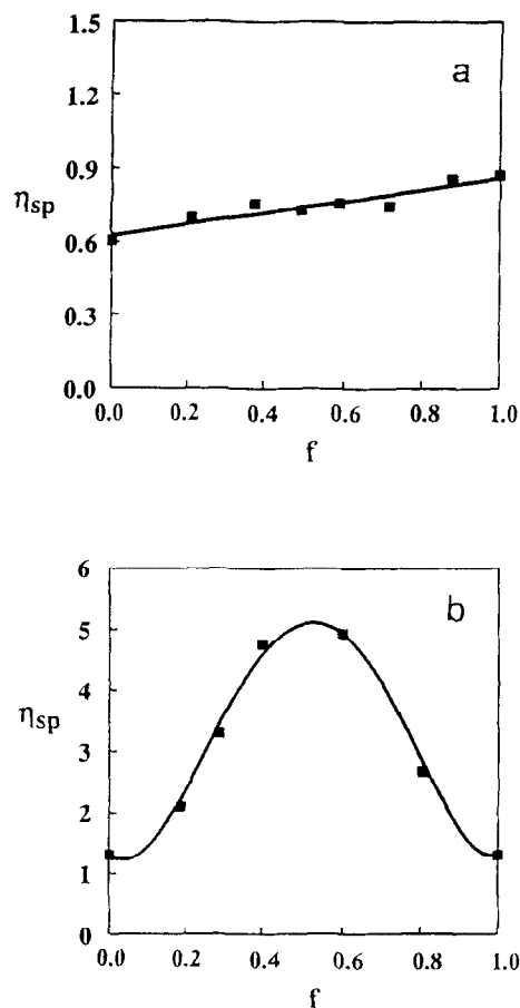
Fig. 2. Specific viscosity (measured at 20°C and 50 s -1 as \dot{\gamma} was increased) for dilute solutions of LBG in combination with (a) lambda carrageenan in 100 mM KCl; and (b) xanthan in 10 mM KCl; f denotes the LBG content expressed as a fraction of the total polymer concentration; the concentrations (% w/w) of the individual polymer solutions were: (a) 0.063 LBG, 0.304 carrageenan; and (b) 0.080 LBG, 0.008 xanthan (as in Fig. 1).
